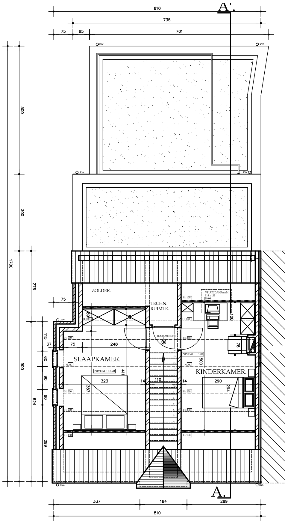
DAKENPLAN.
